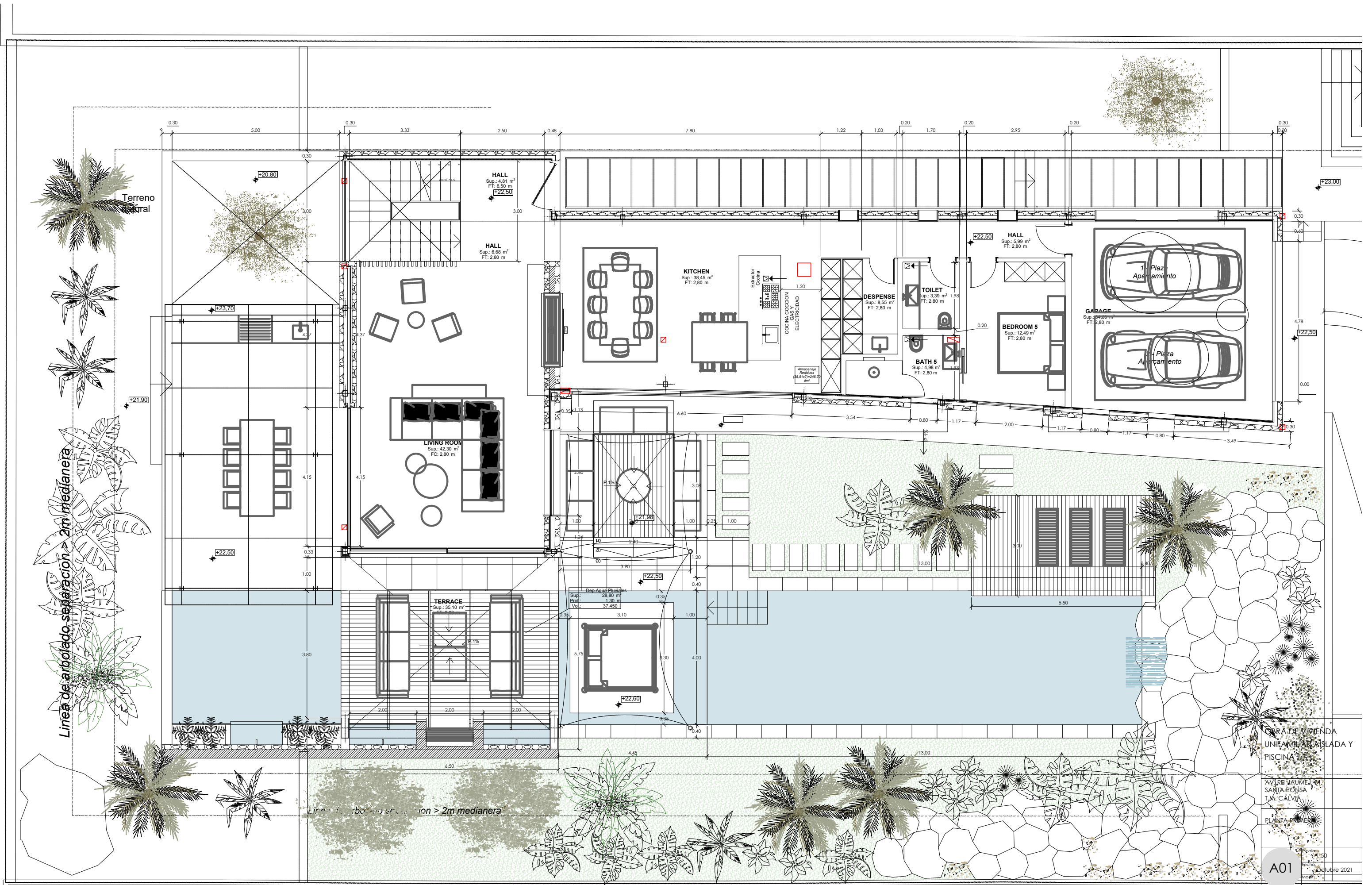
1: 50 GROUND FLOOR
